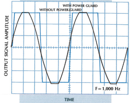
OUTPUT SIGNAL WAVEFORM SHOWING ACTION OF POWER GUARD TO ELIMINATE OUTPUT SIGNAL CLIPPING. POWER AMPLIFIER INPUT IS OVERDRIVEN BY 20 dB FOR BOTH OSCILLOGRAM TRACES.
